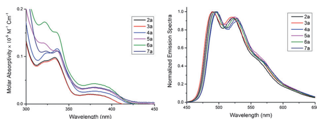
Figure 2. Photophysical data for complexes 2–7a . Top left: UV/Vis absorption spectra in dichloromethane. Top right: Emission spectra measured in degassed CH 2 Cl 2 (10 −5 M) at room temperature.
